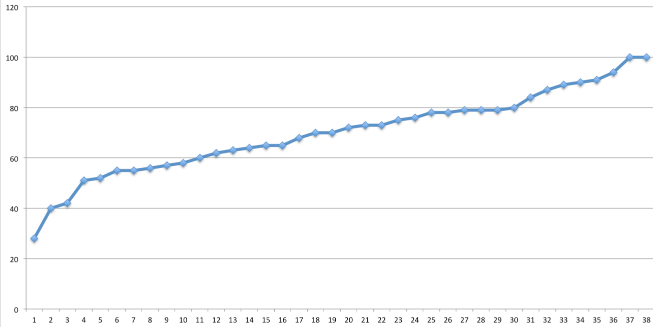
Math 3400 Exam 1 grades
