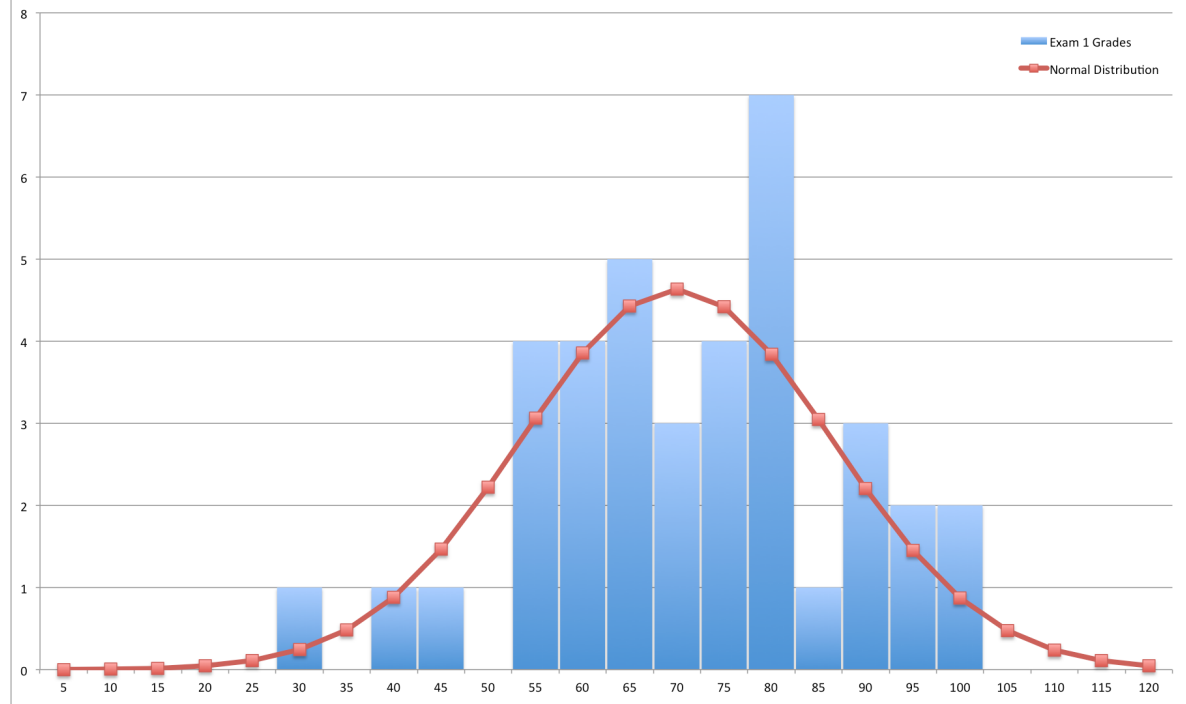
Exam 1 Grade Distribution Math 3400 - Sect 002 - Spring 2016
