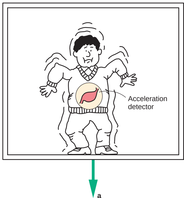
figure 2.8 Your acceleration detector senses the downward acceleration of the elevator.
