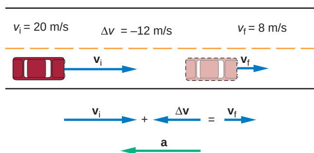
figure 2.11 The velocity and acceleration vectors for decreasing velocity: \Delta \mathbf{v} and \mathbf{a} are now opposite in direction to the velocity. The acceleration \mathbf{a} is proportional to \Delta \mathbf{v} .
