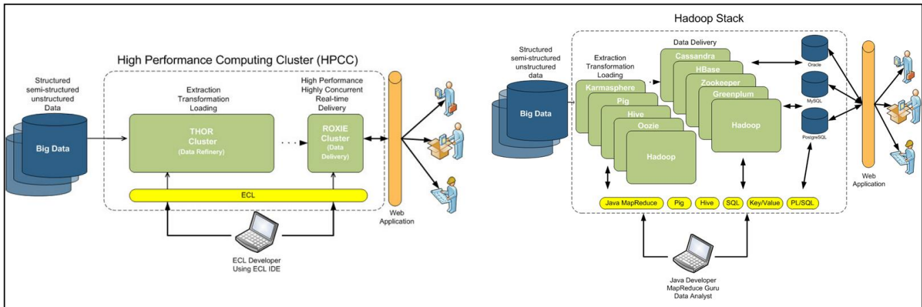
Figure 2. Comparison between HPC Systems Platform and Hadoop architecture [22]
