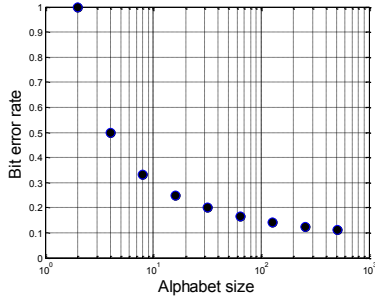
Figure 3: Bit error rate with the bit-to-symbol alphabet size M when correlated jammer dominates
