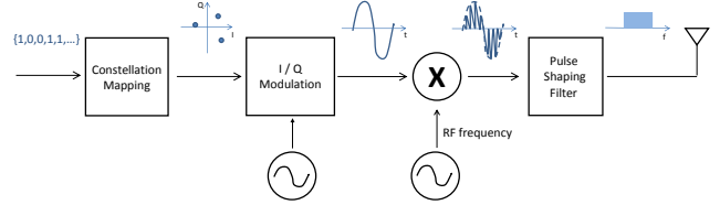
Figure 1: Typical transmitter processing chain at the physical layer
